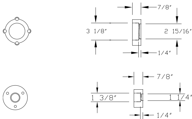
Evaporator Flange Connection. Flange adapter and O-ring supplied by Trane
